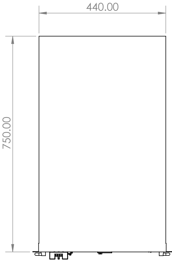
TOP VIEW
